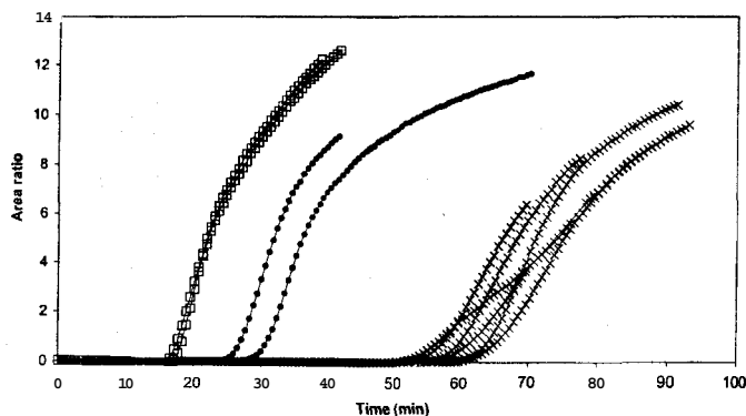
FIG. 9. Effect of temperature on the permeation of acetone through nitrile rubber from a 40% acetone–water mixture using the 1710 \text{cm}^{-1} carbonyl band of acetone ratioed to the 2240 \text{cm}^{-1} band of the nitrile rubber. Replicate experiments at 45 °C (□), 38 °C (●), and 20 °C (×).
