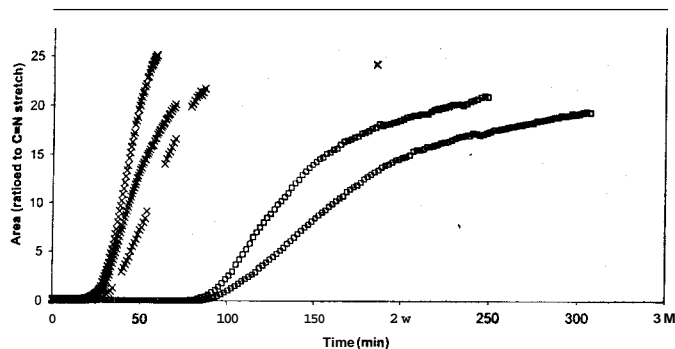
FIG. 11. Comparison of the permeation behaviour, for replicate experiments, of toluene in the malathion concentrate ( \square ) and pure toluene ( \times ) through thick nitrile rubber glove material.
