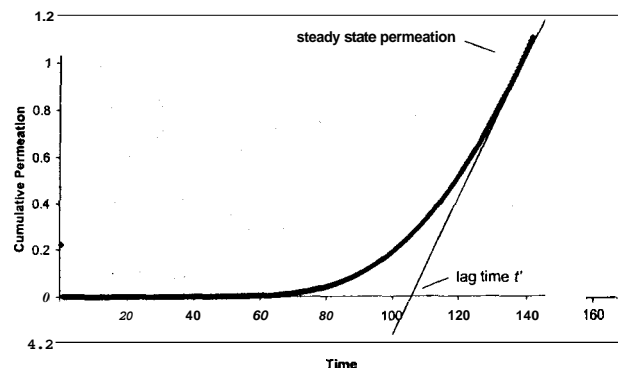
FIG. 10. Example of the measurement of lag time by extrapolation of the linear region of the plot of cumulative permeation vs. time.
