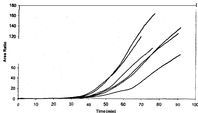
FIG. 6. Ratio of the area of O-H stretching band of water to that of the 2240\text{ cm}^{-1} band of the nitrile rubber for six replicate permeation experiments of a mixture of acetone (40% v/v) and water through nitrile rubber.
