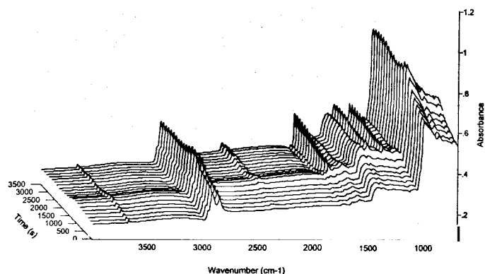
FIG. 2. A typical set of ATR spectra obtained from the permeation of neoprene by acetone.
