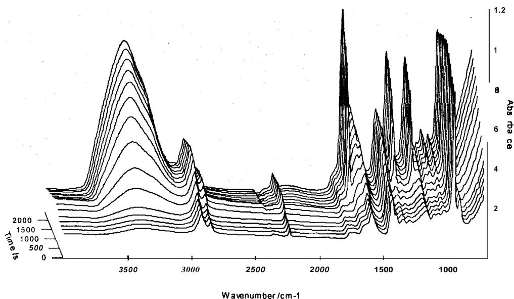
FIG. 4. A typical set of ATR spectra obtained from the permeation of a mixture of acetone (40% v/v) in water through nitrile rubber.
