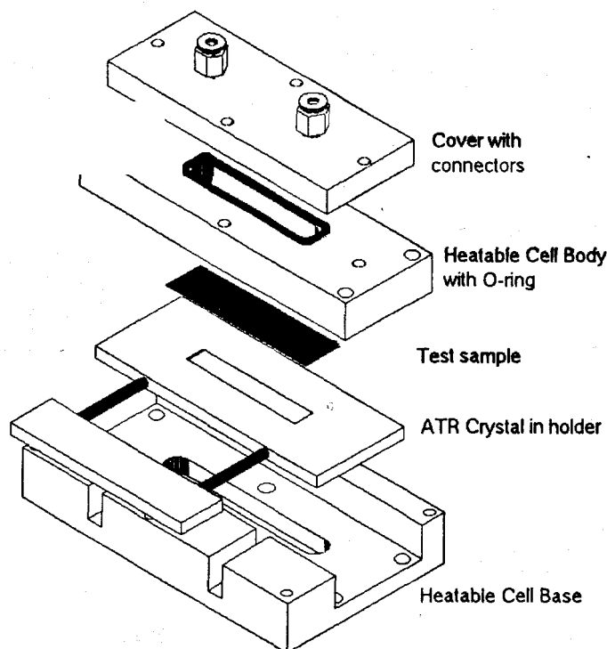
FIG. 1. Schematic diagram of gas-pressurized ATR permeation cell.
