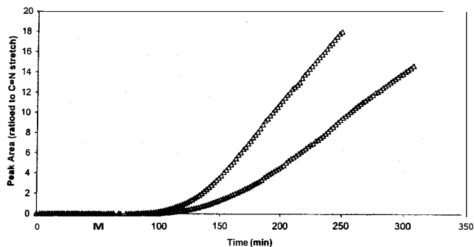
FIG. 12. The permeation behavior, for two replicate experiments, of maldison in malathion concentrate through thick nitrile rubber glove material.
