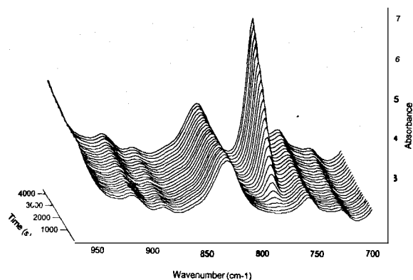
FIG. 7. A typical set of ATR spectra obtained from the permeation of naphthalene through latex.
