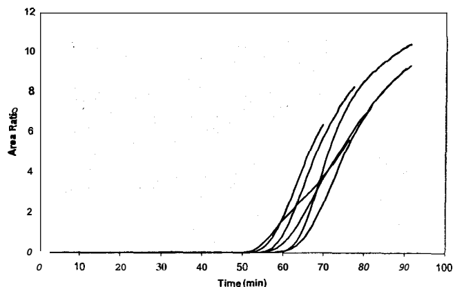
FIG. 5. Ratio of area of the carbonyl band of acetone to that of the 2240\text{ cm}^{-1} band of the nitrile rubber for five replicate permeation experiments of a mixture of acetone (40% v/v) and water through nitrile rubber.
