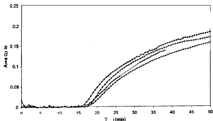
FIG. 3. Area of acetone carbonyl band for four replicate experiments of the permeation of neoprene by acetone, with correction for changing polymer contact by ratioing to the area of the 830 \text{cm}^{-1} neoprene absorption band.
