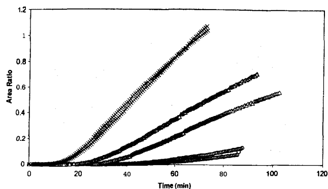
FIG. 8. Effect of temperature on the permeation of naphthalene through thick (0.32 mm) latex glove material by measurement of the 780 \text{cm}^{-1} band. Replicate experiments at 45 °C (x), 38 °C (A), and 20 °C (O).
